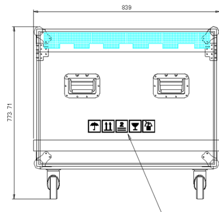
Silk screen printing five-proof logo Symmetrical on both sides
